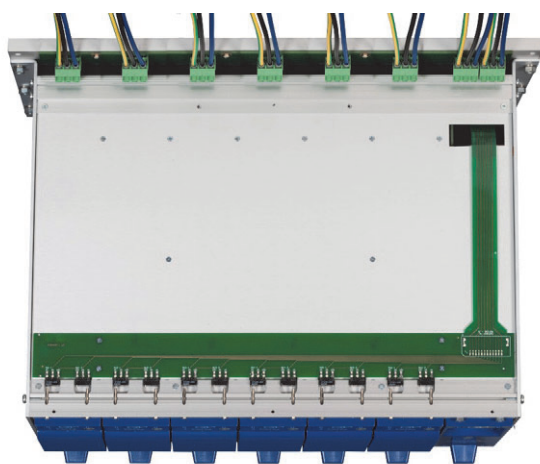
19" Rack Unit type PSR1250-HS-7 Top view without cover
