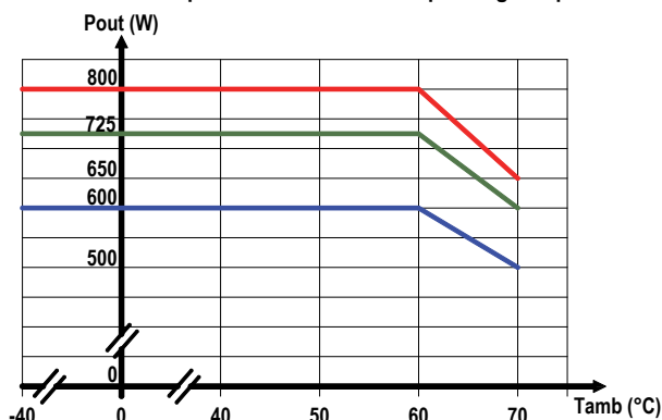
PSW1230 Maximum Output Power vs. Ambient Operating Temperature
