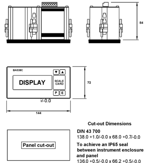
Fig 3 BA538C dimensions
